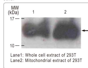
Cytochrome C antibody (GTX108585) WB analysis of Cytochrome C expression in the indicated cell fraction.
