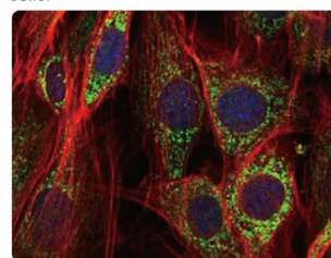
AIF antibody [4E7] (GTX60476) ICC analysis of AIF protein in NIH3T3 cells.
