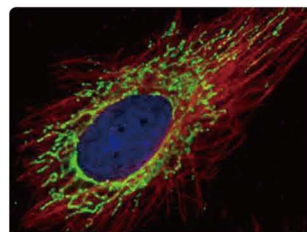
COX4 antibody (GTX101499) ICC analysis of COX4 protein in HeLa cells.
