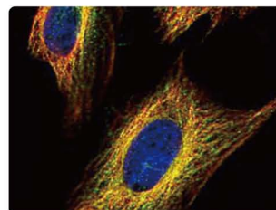
VDAC2 antibody [C2C3], C-term (GTX104745) ICC analysis of VDAC2 protein in HeLa cells.
