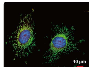
FIS1 antibody [GT9810] (GTX631209) ICC analysis of FIS1 protein in HeLa cells.
